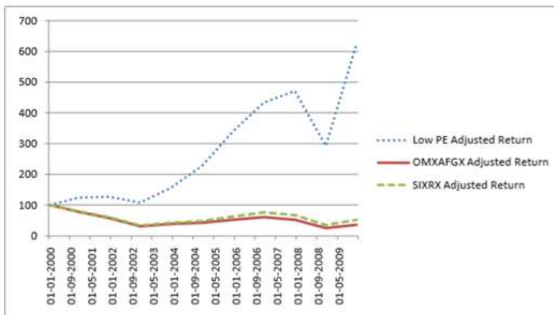
Gráfico 2: Low P/E portfolio, OMXAFGX y SIXRX index accumulated risk adjusted return for periods (2000-2009)
